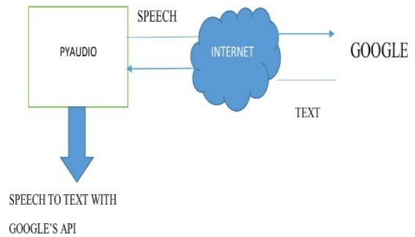
Fig.5: Google Speech-to-text
