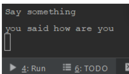
Fig.4: Speech Input
