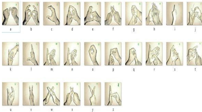
Fig.2: Predefined signs
