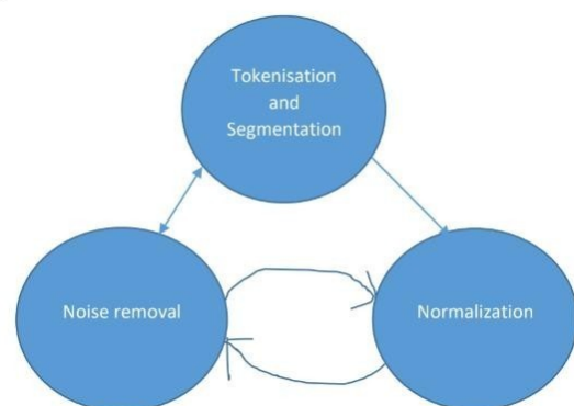
Fig.6: Text pre-processing
